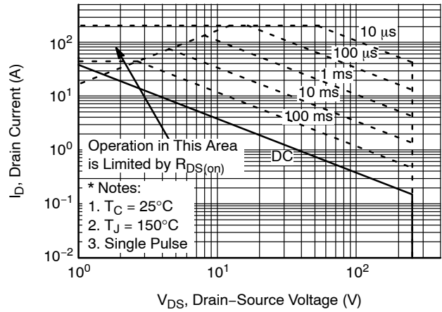
Figure 9-2. Maximum Safe Operating Area for FDPF51N25
